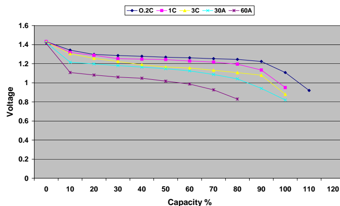
Discharging Curve
